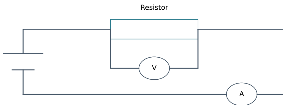
DC supply in series
