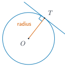
tangent meets radius = 90^\circ
