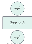
Cylinder net 2 circles + a rectangle
