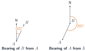
Bearing of B from A
