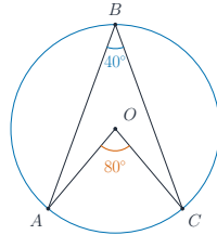
angle at centre = 2 \times angle at circumference
