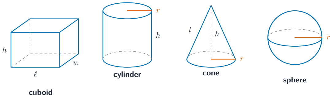
Common solids and the dimensions ( r , h , \ell , slant l ) used in their volume and surface-area formulas.
