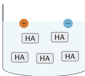
weak acid mostly molecules, few ions (e.g. ethanoic acid)
