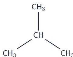
2-methylpropane (branched)
