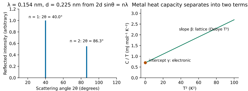
Bragg diffraction and electron-gas heat capacity: original GRE teaching diagram.
