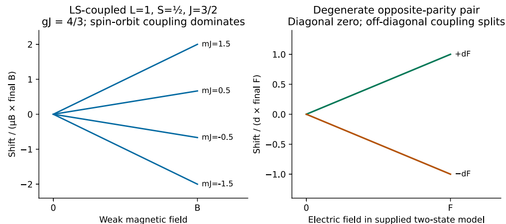
Atomic spectra and selection rules: original GRE teaching diagram.
