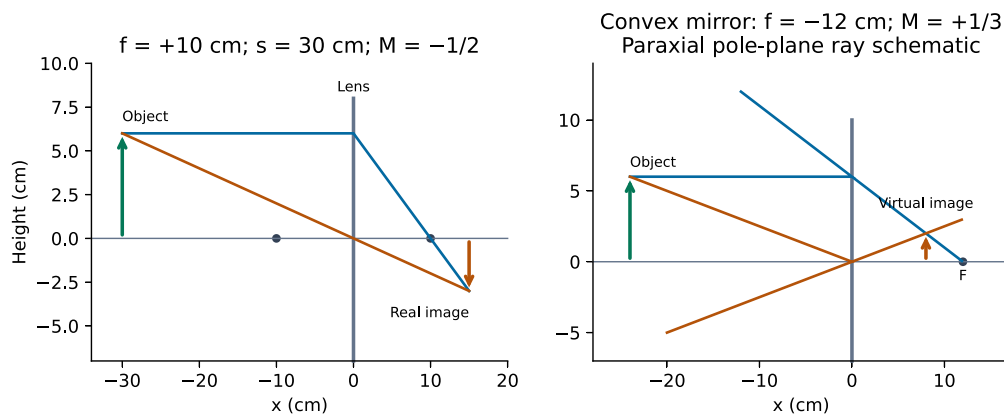
Signed lens and mirror images: original GRE teaching diagram.
