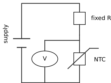
Output across lower thermistor
