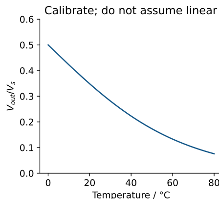
Output across lower thermistor
