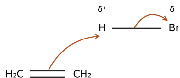
1 Form the ethyl carbocation
