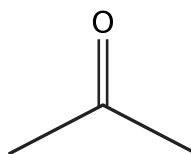
Skeletal formula
