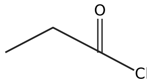
Skeletal formula
