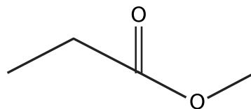
Skeletal formula
