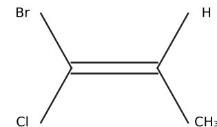
B: E (Br and CH_3 apart)
