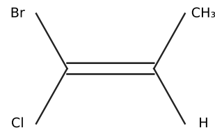
A: Z (Br and CH_3 together)
