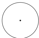
s orbital: spherical
