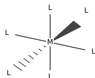
Octahedral: six donors
