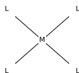
Square planar: four donors
