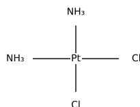
Cisplatin: adjacent Cl
