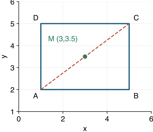
Coordinate rectangle: lengths 4 and 3; diagonal 5
