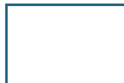
Side: 3 \times 2
