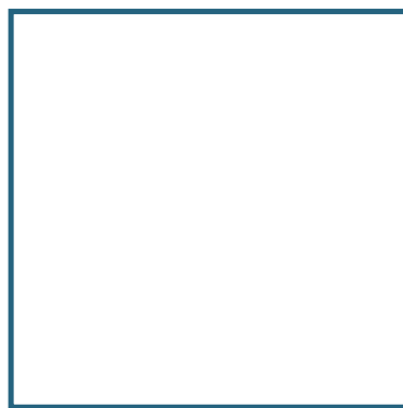
length 3; area 9
