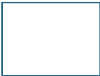
Plan: 4 \times 3
