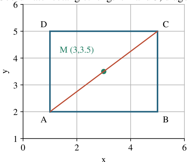
Coordinate rectangle: lengths 4 and 3; diagonal 5
