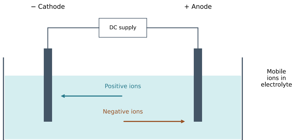
Powered electrolysis: electrodes kept apart; electrons travel in external circuit
