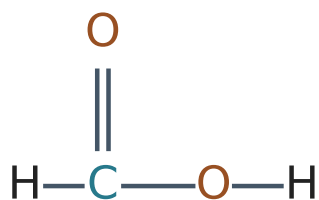
Methanoic acid
