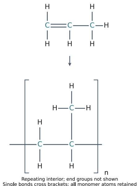
Propene monomer
