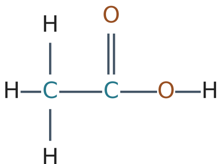
Ethanoic acid
