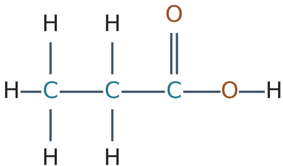
Propanoic acid
