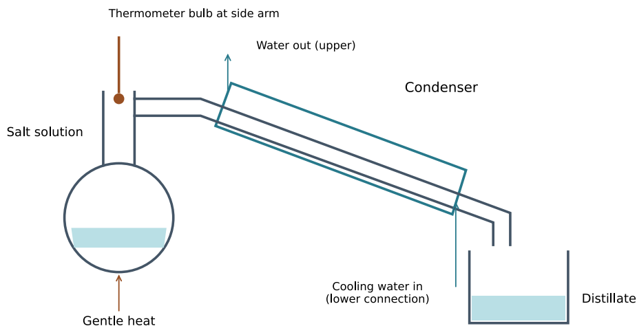
Simple distillation: open receiving path; salt stays in the flask
