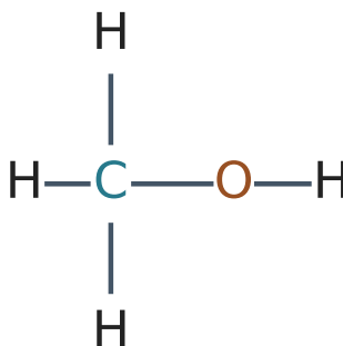
Methanol
