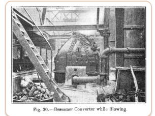
Fig. 30.—Bessemer Converter while Blowing. a Bessemer converter blowing
