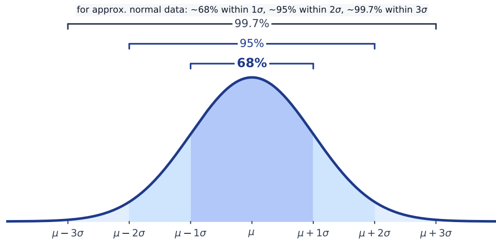
The normal curve and the 68-95-99.7 empirical rule
