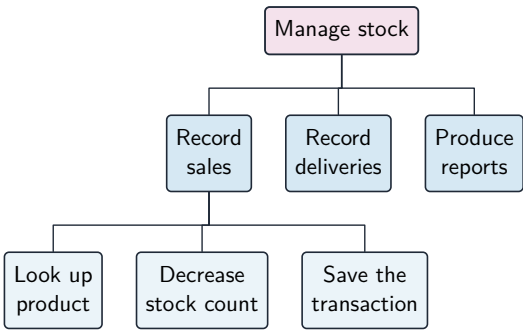
Decomposing a program into procedures and sub-procedures
