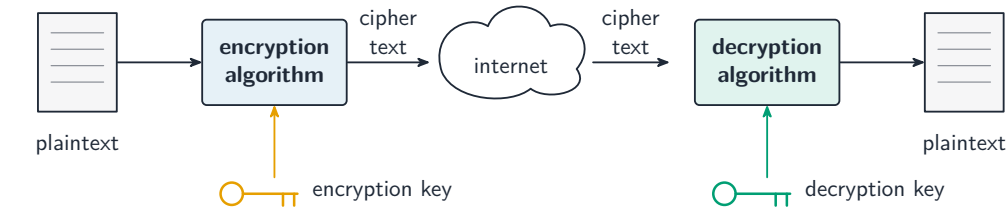
Encryption scrambles plaintext with a key; only the key can decrypt it
