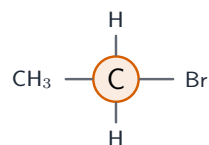
primary 1 C on the C-Br carbon
