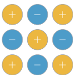
giant ionic NaCl: high m.p., conducts when molten
