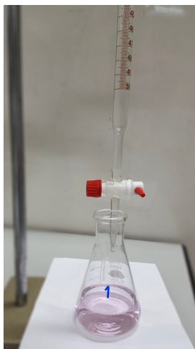
A titration finds reacting volumes precisely.
