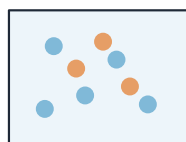
homogeneous (same state, mixed in)
