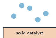
heterogeneous (different state, a surface)
