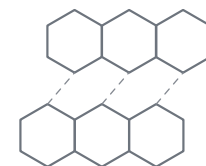
graphite layers slide; spare electrons let it conduct
