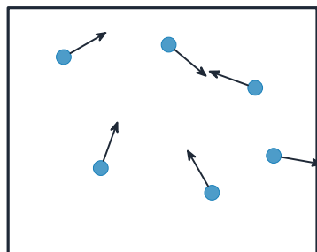
ideal gas (model) point particles, no forces
