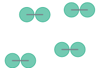
simple molecular I 2 , ice: low m.p., weak forces between
