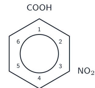
3-nitrobenzoic acid
