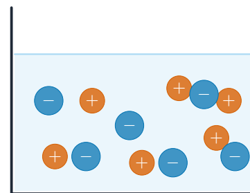
strong acid fully dissociated: many ions
