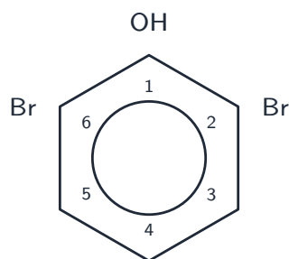
2,4,6-tribromophenol
