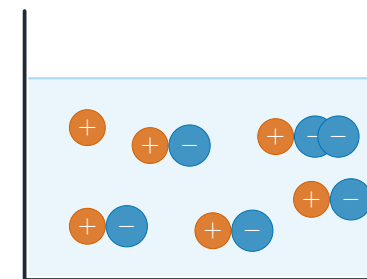
weak acid mostly molecules: few ions
