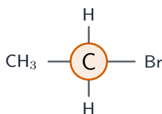
primary 1 C on the C–Br carbon
