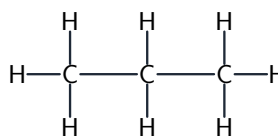
propane \text{C}_3\text{H}_8
