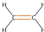
ethene \text{C}_2\text{H}_4 unsaturated: \text{C}=\text{C} double bond
