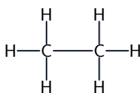
ethane \text{C}_2\text{H}_6
