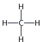
methane \text{CH}_4
