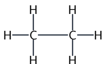
ethane \text{C}_2\text{H}_6 saturated: single \text{C}-\text{C} bond
